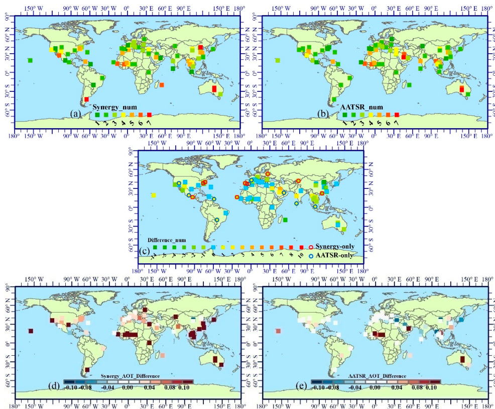
Figure A2. Global spatial distribution of collocated pairs and the AOT difference between SU/synergy AOT and SU/AATSR AOT with AERONET datasets for each site in March 2008. Spatial distributions of (a) synergy collocated pairs, (b) AATSR collocated pairs, (c) the synergy collocated pairs difference, (d) the synergy AOT difference (synergy AOT—AERONET AOT), and (e) the AATSR AOT difference (AATSR AOT—AERONET AOT).
