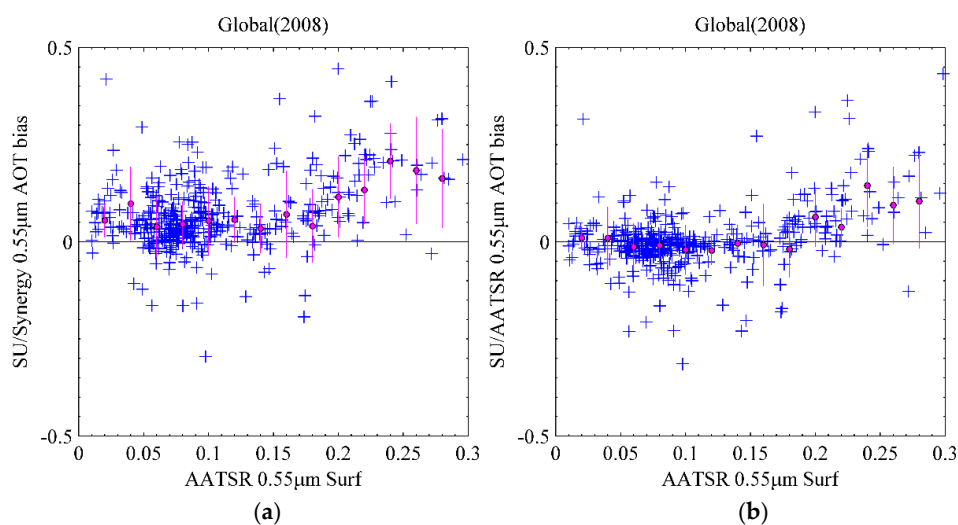
Figure 10. Scatter plots of SU/synergy (a) and SU/AATSR (b) bias with respect to SU/AATSR surface reflectance in the 550 nm wavelength. The magenta circles represent the means of AOT differences in each range and lines of the same color represent the means \pm \sigma .
