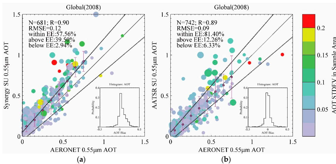
Figure 7. Scatter plots of AERONET L2 data with (a) SU/synergy and (b) SU/AATSR L2 AOT products in 2008. The colors of each point represent the AOT standard deviation in a sampling area measuring 50 \times 50 km. Areas of each point represent the uncertainties of satellite retrieval (provided in the dataset) for each collocated pair. The magenta points and lines are the mean and mean \pm 2\sigma of satellite retrieved AOTs in each AERONET AOT range (0.1). The dashed bold lines stand for expected error (EE) of \pm 0.15AOT_{AERONET} \pm 0.05 .
