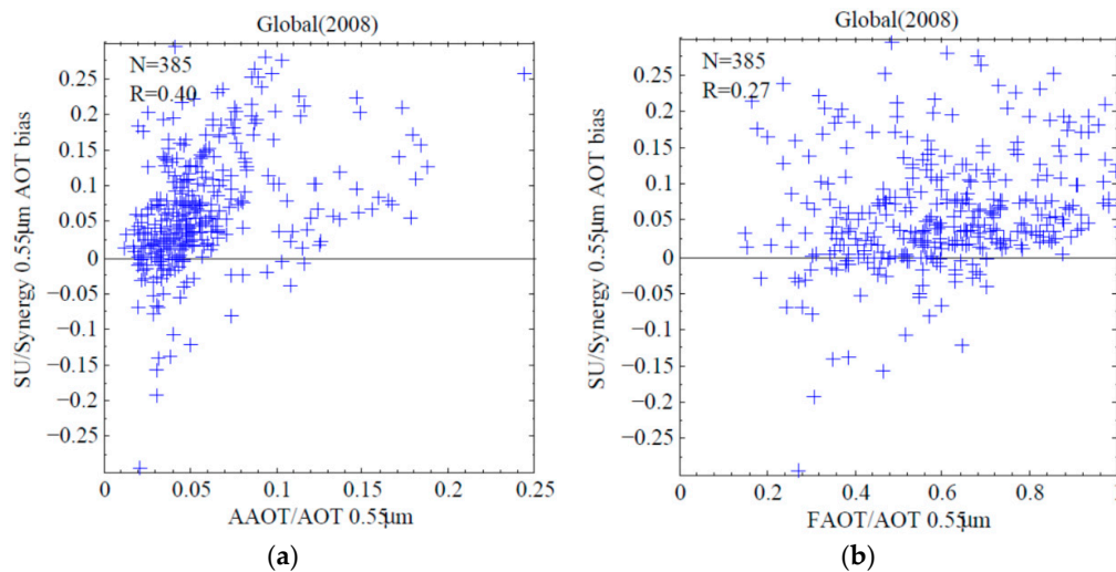
Figure 12. Scatter plots of (a) absorption aerosols/AERONET AOT with SU/synergy AOT bias and (b) fine-mode aerosols/AERONET AOT with SU/synergy AOT bias.
