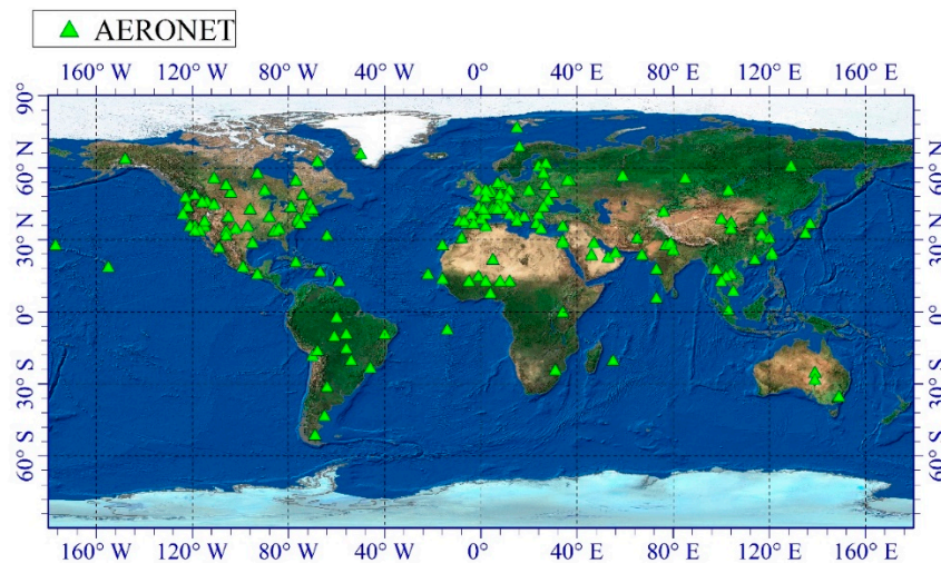
Figure 1. The spatial distribution of AERONET sites (green) used for validation.
