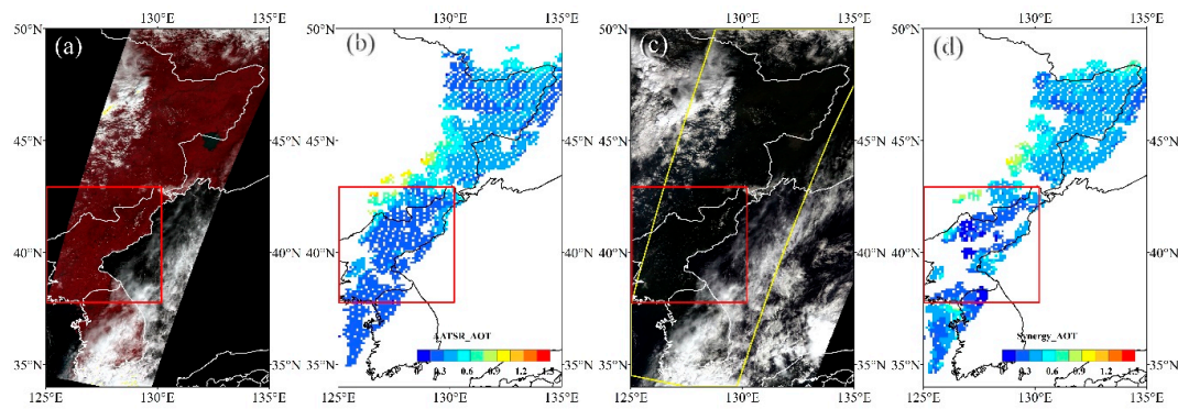
Figure 9. Influence of cloud masking in China and Korea: (a) AATSR RGB map, (b) SU/AATSR AOT, (c) MERIS RGB map, and (d) SU/synergy AOT.
