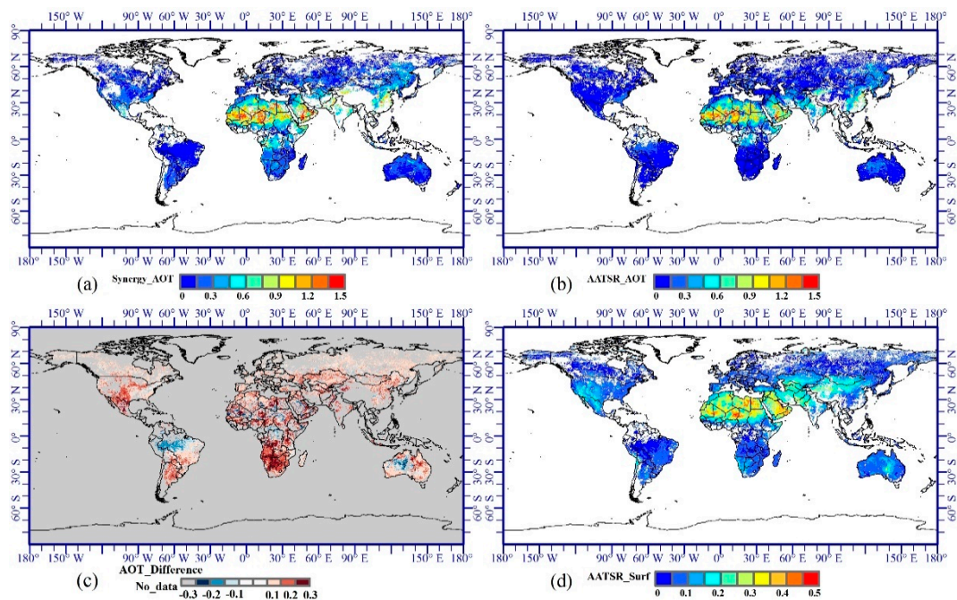
Figure 3. Global averaged monthly AOT difference between SU/synergy and SU/AATSR in June 2008. (a) Synergy AOT, (b) AATSR AOT, (c) AOT difference (synergy—AATSR), and (d) AATSR surface reflectance.
