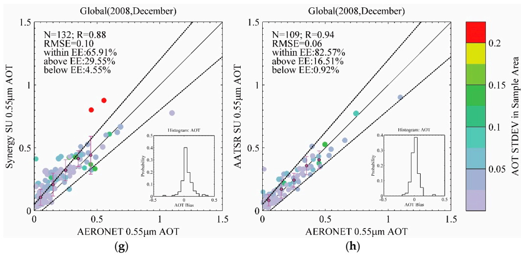
Figure A1. Seasonal (March, June, September, and December) scattering plots of AERONET data with SU/synergy and SU/AATSR data, 2008. (a) synergy AOT vs. AERONET AOT in March, (b) AATSR AOT vs. AERONET AOT in March, (c) synergy AOT vs. AERONET AOT in June, (d) AATSR AOT vs. AERONET AOT in June, (e) synergy AOT vs. AERONET AOT in September, (f) AATSR AOT vs. AERONET AOT in September, (g) synergy AOT vs. AERONET AOT in December, and (h) AATSR AOT vs. AERONET AOT in December.
