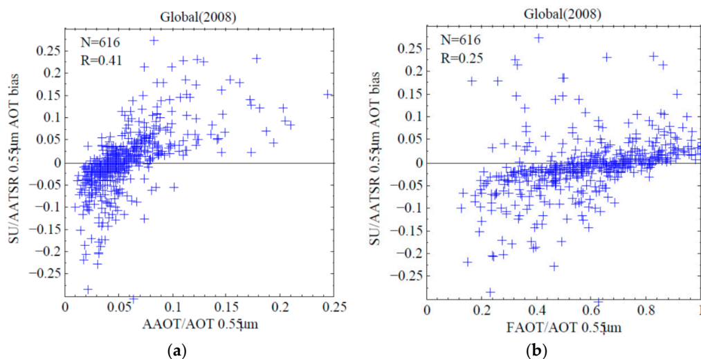
Figure 13. Scatter plots of (a) absorption aerosols/AERONET AOT with SU/AATSR AOT bias and (b) fine-mode aerosols/AERONET AOT with SU/AATSR AOT bias.
