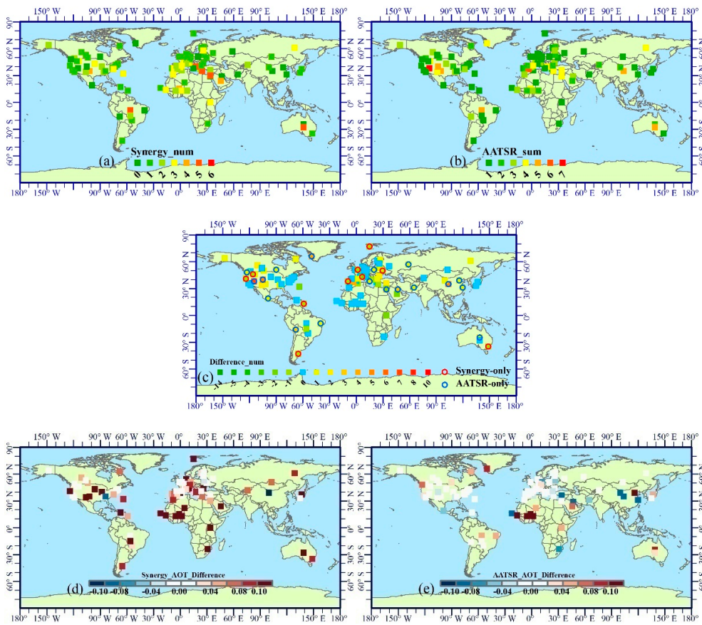
Figure A3. Global spatial distribution of collocated pairs and the AOT difference between SU/synergy AOT and SU/AATSR AOT with AERONET datasets for each site in June 2008. Spatial distributions of (a) synergy collocated pairs, (b) AATSR collocated pairs, (c) the synergy collocated pairs difference, (d) the synergy AOT difference (synergy AOT—AERONET AOT), and (e) the AATSR AOT difference (AATSR AOT—AERONET AOT).
