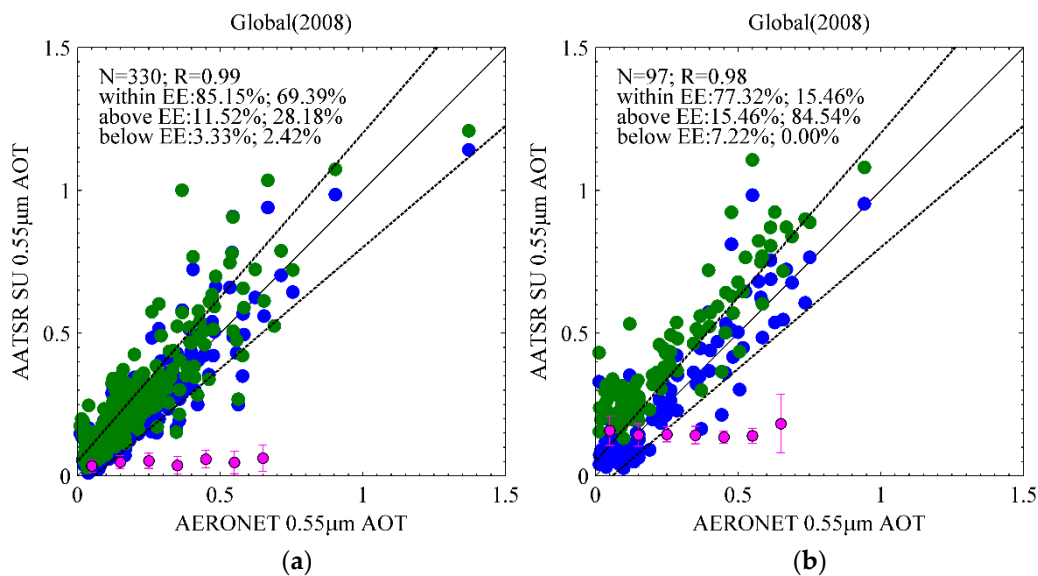
Figure 8. Scatter plot of SU/synergy AOT and SU/AATSR AOT with AERONET data for AOT \leq bias < 0.1 (a) and AOT bias > 0.1 (b). Blue points represent SU/AATSR AOTs and green points represent SU/synergy AOTs. The magenta circles are the means of AOT difference in each range and lines of the same color are the means \pm \sigma . The dashed bold lines stand for expected error (EE) of \pm 0.15AOT_{AERONET} \pm 0.05 .
